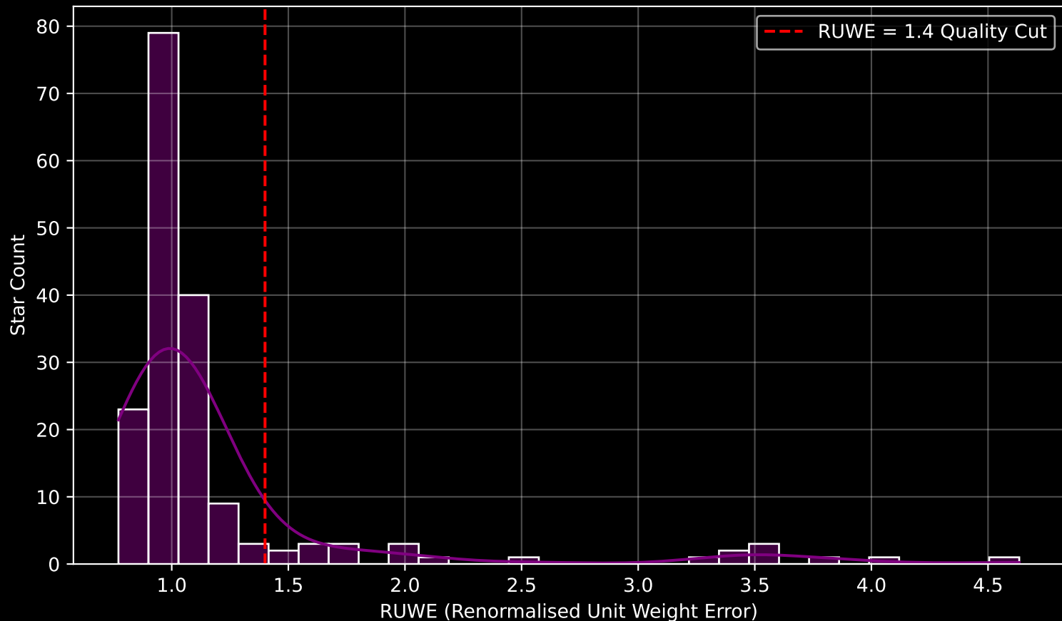
GAPOGEE DR17 Field [115+66_MGA] RUWE Distribution (n= 176)
