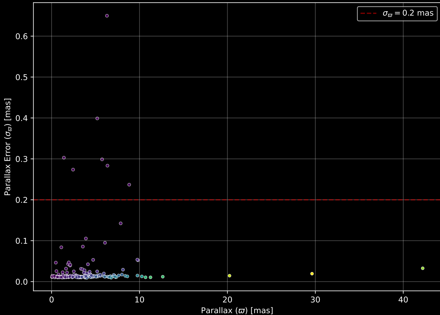
APOGEE DR17 Field: [115+66_MGA] Parallax Quality (n= 188)
