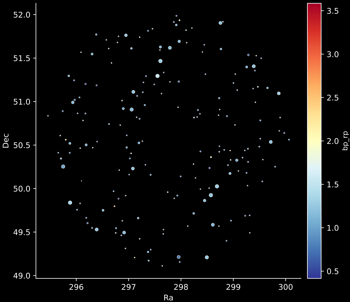
APOGEE DR17 Field: [115+66_MGA] Stars: 188
