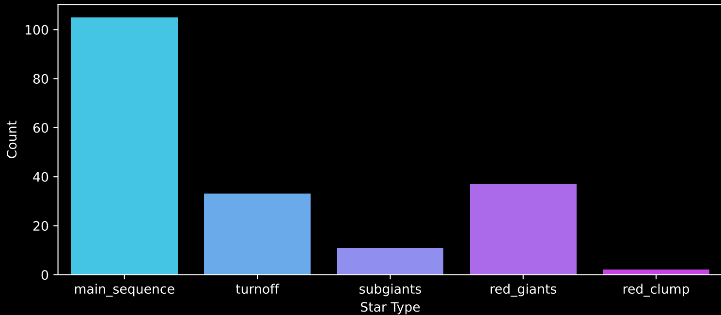
APOGEE DR17 Field: [115+66_MGA] Count plot of Star Type
