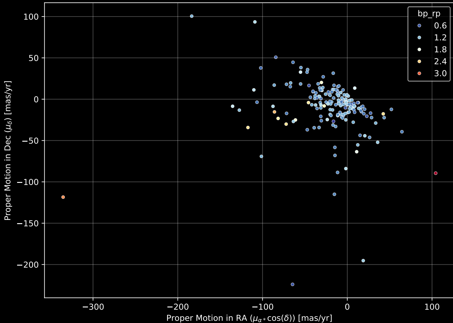
APOGEE DR17 Field: [115+66_MGA] Proper Motion Diagram (n= 188)
