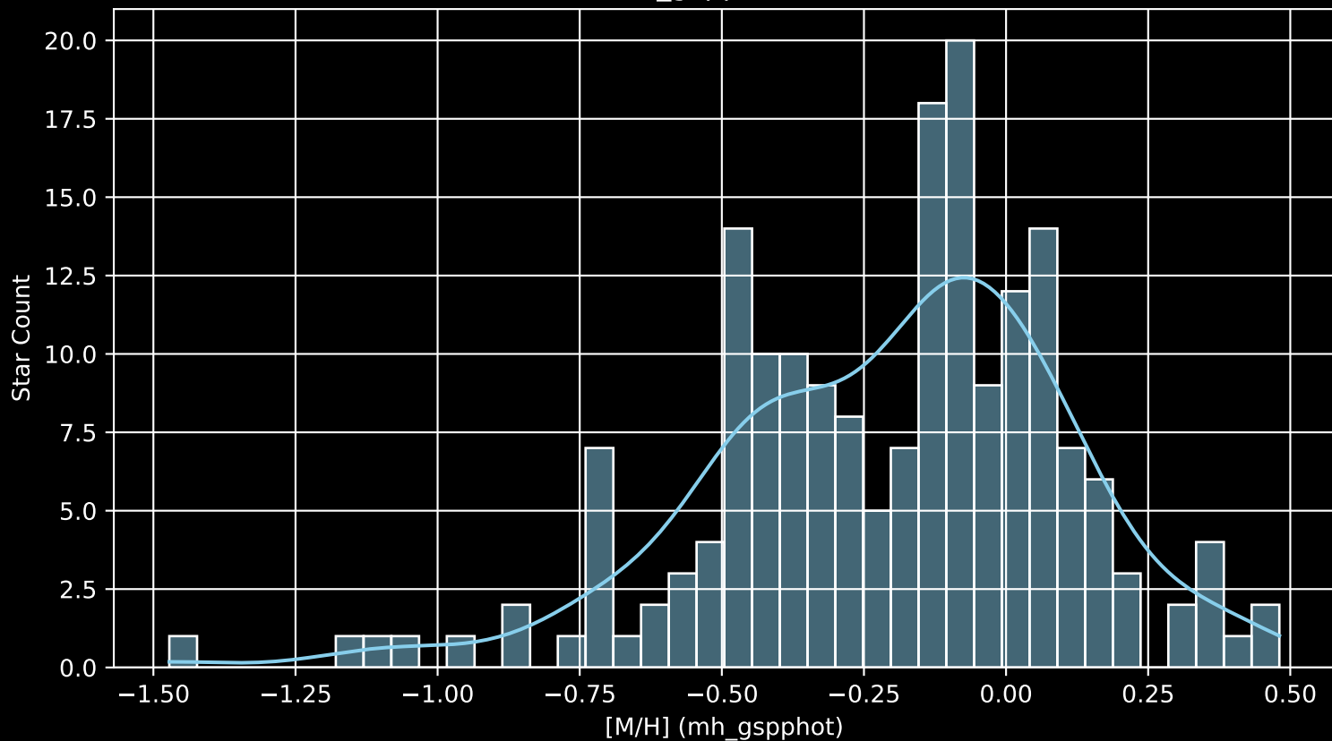
APOGEE DR17 Field: [115+66_MGA [M/H] (mh_gspphot) (n= 186)
