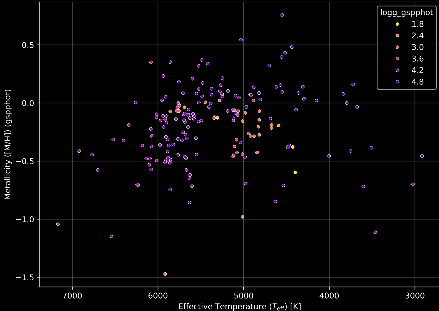
APOGEE DR17 Field: [115+66_MGA] Stellar Population Parameters (n= 188)
